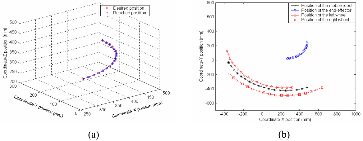
Fig.3. The simulation results of opening a door with real working range for manipulator joints. (a) gives the desired and reached positions of the end-effector in the world frame in 3D space. (b) shows the positions of frame O_m of the mobile base, the positions of the wheels, and the positions of the end-effector in the world frame in 2D. gripper opened the door, its trajectory was a piece of circle arc.
