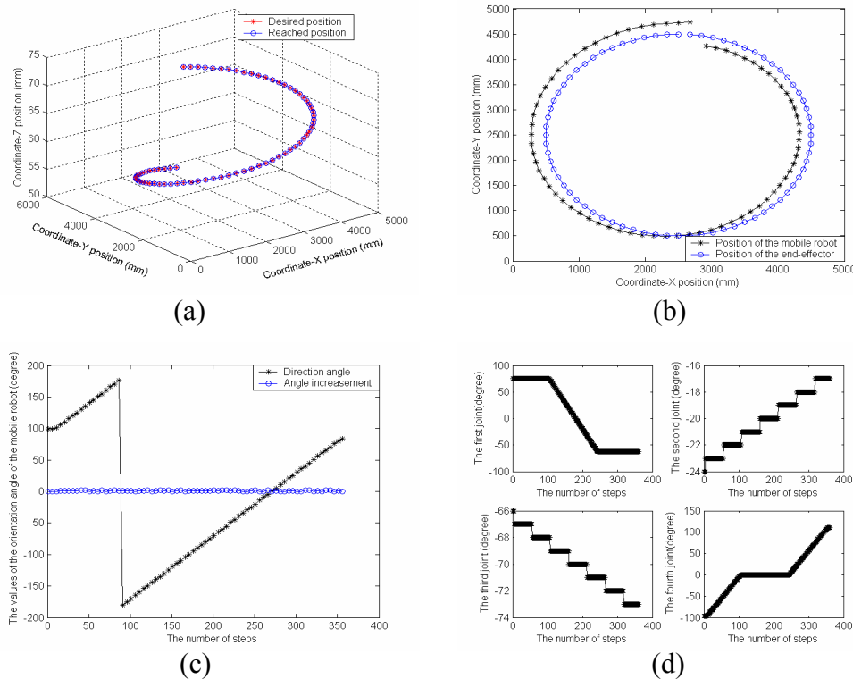
Fig.2. The results of the 1st simulation with real working range for manipulator joints. (a) gives the desired and reached positions of the end-effector in the world frame in 3D space. (b) shows the positions of frame O_m of the mobile base, and the positions of the end-effector in the world frame. The direction angles of the mobile base and their increments are shown in (c). The values of joint angles of the manipulator are shown in (d).
