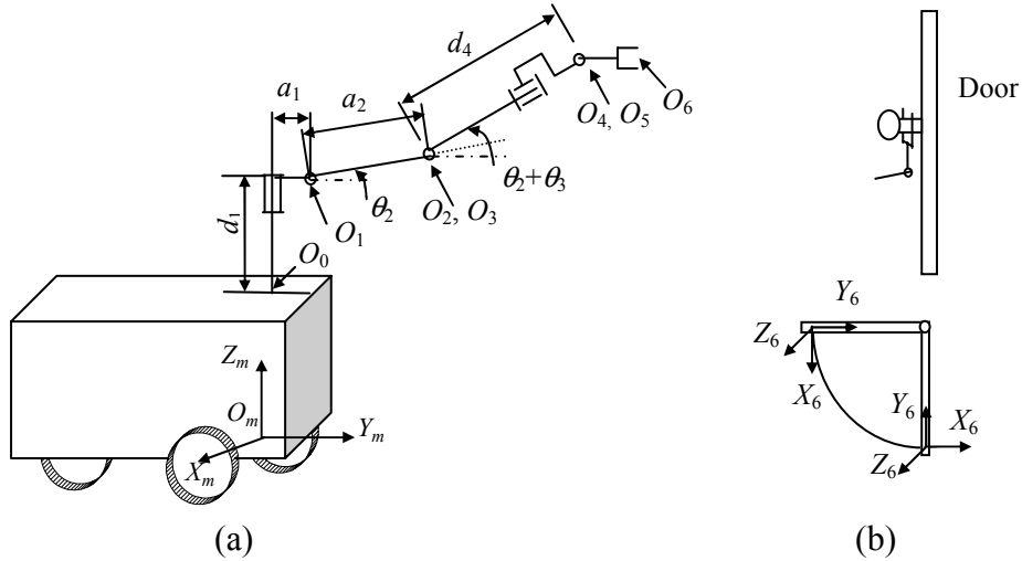
Fig.1. The mobile manipulator and its task. The configuration sketch of the mobile manipulator is shown in (a). The principle sketch of opening a door is shown in (b).
