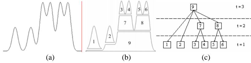
Fig 3 An example of Peak Analysis . (a) 1D profile of the original image; (b) its peaks; (c) the tree to store the result of the analyzed peaks
