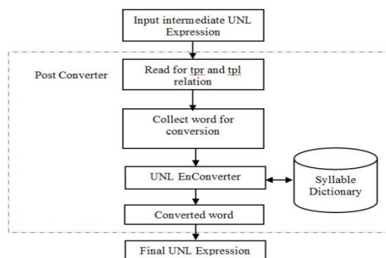
Figure 5. Architecture of Post converter (Bengali to English)
